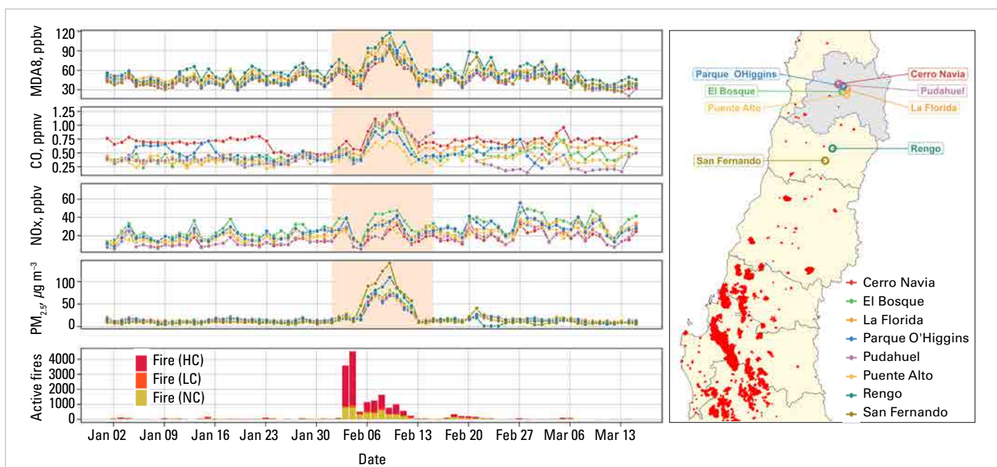
Figure 10. Time series of the maximum daily 8-hour average (MDA8) ozone, carbon monoxide (CO) (in parts per million (ppmv)), nitrogen oxides (NOx) and fine particulate matter ( PM_{2.5} ) from selected air quality monitoring stations (MDA8>50 ppbv) for the period January to March 2023. The lower panel shows the daily (24 h) active fires obtained from MODIS satellite products ( https://modis-fire.umd.edu ) at 1 km resolution (MOD13A1), with coloured bars indicating confidence (high (HC), nominal (NC) and low (LC)) based on infrared radiation emission. The map (right panel) shows the active fires during February in central Chile. The Santiago Metropolitan Region, where most of the monitoring stations are located, is shaded grey.
