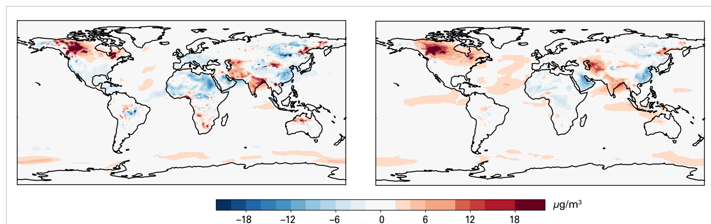
Figure 1. PM_{2.5} anomaly ( \mu g\ m^{-3} ) in 2023 (reference period 2003–2022)
