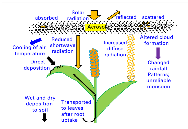
Figure 4. The multiple routes by which PM affects crops, including direct deposition to crop leaves and soil (black arrows), and indirect impacts via effects on sunlight (solar, short-wave and diffuse radiation: orange arrows), temperature (blue arrow) and rainfall (purple arrow)
